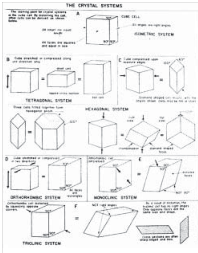
Fig. 6-34. Crystal systems.
